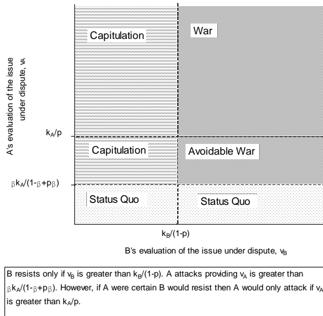
Figure 2: The Outcome in the Crisis Game given the type of each player
