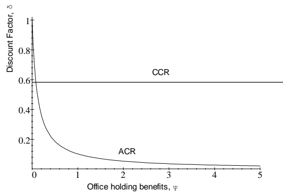
Figure 3: The minimum discount factor to ensure fully credible foreign policy statements under the Country Contingent Reputation and the Agent Contingent Reputation Strategies.
