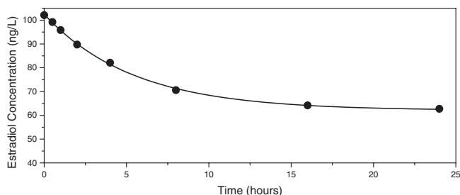
Figure 4 Static adsorption of estradiol onto the NF-270 membrane (feed solution: 100 ng/L estradiol, 1 mM NaHCO 3 , 20 mM NaCl, and pH 8.0)
