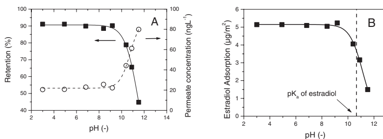
Figure 1 pH effect on permeate concentration, retention, and adsorption of estradiol by the TFC-SR2 membrane (feed solution: 100 ng/L estradiol, 1 mM NaHCO 3 , 20 mM NaCl)
