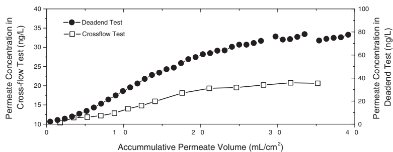
Figure 3 Permeate concentration of estrone in dead end and crossflow filtration with the TFC-S membrane as a function of permeate volume (feed solution: 100 ng/L estrone, 1 mM NaHCO 3 , 20 mM NaCl, and pH 8.0)
