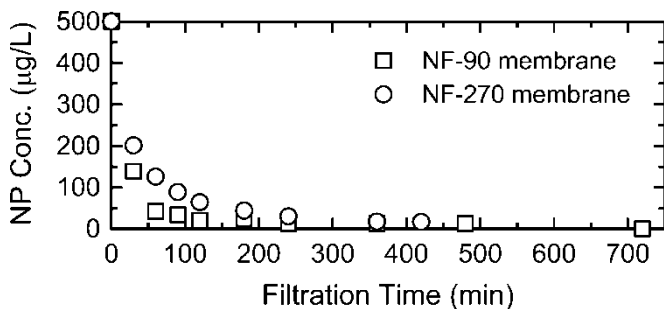
Figure 4. Feed concentrations of nonylphenol (NP) as a function of filtration time for the NF-90 and NF-270 membranes. The feed solution contained approximately 500 \mu\text{g/L} of NP in deionized water. Other experimental conditions were as follows: cross-flow velocity = 30.4 cm/s, permeate flux = 15 \mu\text{m/s} (54 \text{L/m}^2\text{h} ), pH = 6, and temperature = 20.0°C. The permeate and retentate were recirculated back to the feed reservoir during the nanofiltration run.
