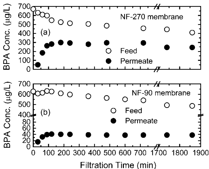
Figure 2. Permeate and feed concentrations of bisphenol A (BPA) as a function of filtration time for the (a) NF-270 and (b) NF-90 membranes. The feed solution contained approximately 500 \mu\text{g/L} of BPA in deionized water. Other experimental conditions were as follows: cross-flow velocity = 30.4 \text{ cm/s} , permeate flux = 15 \mu\text{m/s} ( 54 \text{ L/m}^2 \text{ h} ), \text{pH} = 6 , and temperature = 20.0^\circ\text{C} . The permeate and retentate were recirculated back to the feed reservoir during the nanofiltration run.
