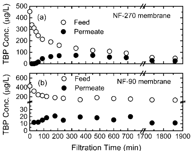
Figure 3. Permeate and feed concentrations of tert-butylphenol (TBP) for the (a) NF-270 and (b) NF-90 membranes. The feed solution contained approximately 500 \mu\text{g/L} of TBP in deionized water. Other experimental conditions were as follows: cross-flow velocity = 30.4 cm/s, permeate flux = 15 \mu\text{m/s} (54 \text{L/m}^2\text{h} ), pH = 6, and temperature = 20.0°C. The permeate and retentate were recirculated back to the feed reservoir during the nanofiltration run.
