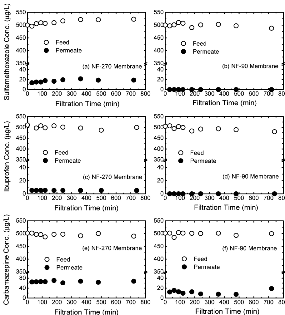
FIGURE 5. Permeate and feed concentrations of sulfamethoxazole, ibuprofen, and carbamazepine as a function of filtration time for the NF-270 and NF-90 membranes. The feed solution contained 500 µg/L of the corresponding pharmaceutical in a background electrolyte solution containing 20 mM NaCl and 1 mM NaHCO 3 . Other experimental conditions were as follows: cross-flow velocity = 30.4 cm/s, permeate flux = 15 µm/s (54 L m -2 h -1 ), pH = 8, temperature = 20 °C. The permeate and retentate were recirculated back to the feed reservoir during the nanofiltration run.
