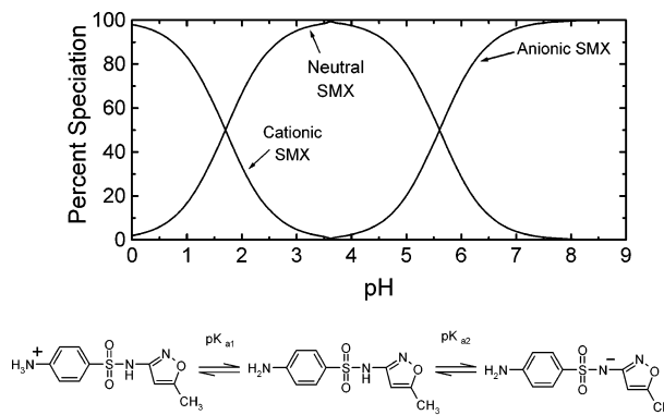
FIGURE 4. Speciation of sulfamethoxazole as a function of pH, calculated based on the pK_a values in Table 1.
