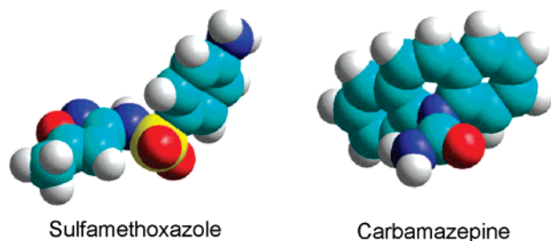
FIGURE 7. Three-dimensional model of sulfamethoxazole and carbamazepine, simulated using HyperChem 7.0 (31).
