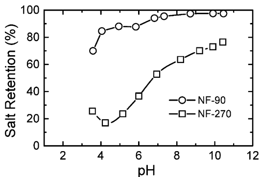
FIGURE 3. Salt retention (measured by electric conductivity) by the NF-90 and NF-270 membranes as a function of pH. The feed solution contained 20 mM NaCl and 1 mM NaHCO 3 .
