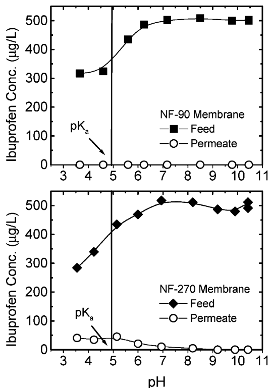
FIGURE 8. Feed and permeate concentration of ibuprofen as a function of the solution pH for the NF-90 membrane (top) and NF-270 membrane (bottom). The feed solution contained 500 µg/L of ibuprofen in a background electrolyte solution containing 20 mM NaCl and 1 mM NaHCO 3 . After each pH adjustment, the system was equilibrated for 1 h prior to sample collection for analysis. Other experimental conditions were as follows: cross-flow velocity = 30.4 cm/s, permeate flux = 15 µm/s (54 L m -2 h -1 ), temperature = 20 °C. The permeate and retentate were recirculated back to the feed reservoir during the nanofiltration run.
