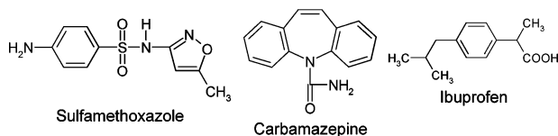
FIGURE 1. Chemical structures of the three pharmaceuticals used in this study. Physicochemical properties of the compounds are described later in Table 1.
