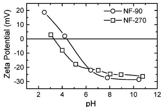
FIGURE 2. Zeta potential of the NF-90 and NF-270 membranes as a function of pH in a background electrolyte solution containing 20 mM NaCl and 1 mM NaHCO 3 .
