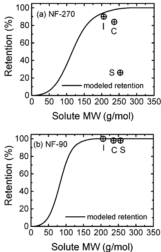
FIGURE 9. Measured retention values of the three pharmaceuticals (open symbols)—sulfamethoxazole (S), carbamazepine (C), and ibuprofen (I)—compared to model predictions (solid line), presented in our previous publication (22) for retention of nonadsorptive inert organics as a function of solute molecular weight: (a) NF-270, (b) NF-90. The retentions of these pharmaceuticals were measured at approximately pH 3.5, where the compounds are neutrally charged (Figure 6). Parameters used in the pore transport model predictions were as follows: cross-flow velocity = 30.4 cm/s, permeate flux = 15 µm/s (54 L m -2 h -1 ), temperature = 20 °C.
